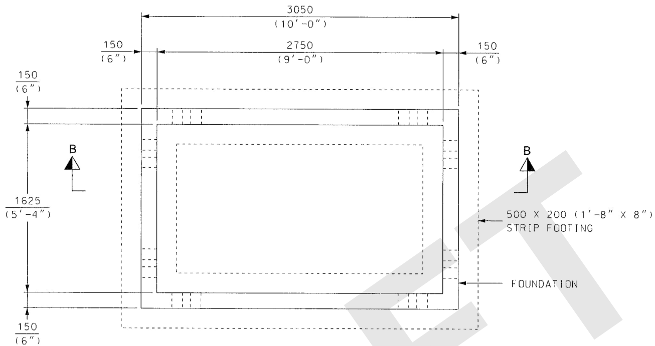
PRECAST OPTION ⚠ PLAN VIEW
