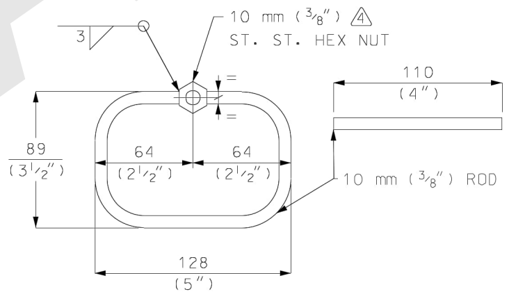
DETAIL 'D'
