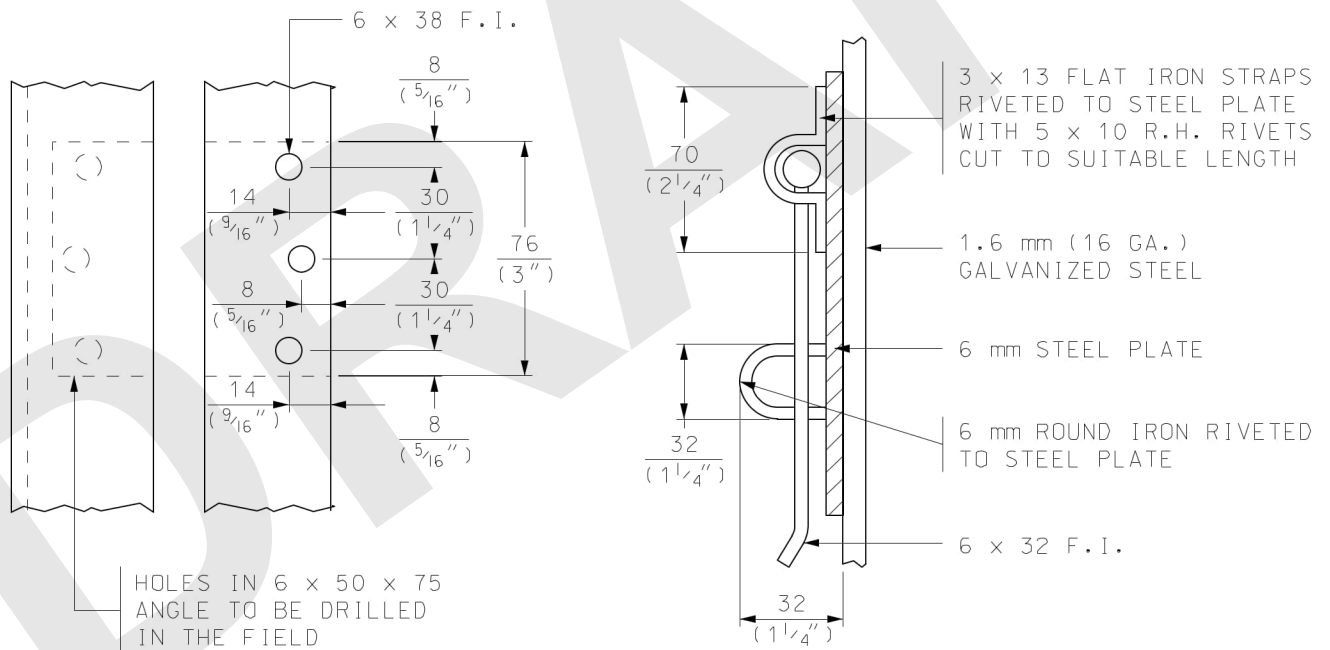
DETAIL OF HINGE
