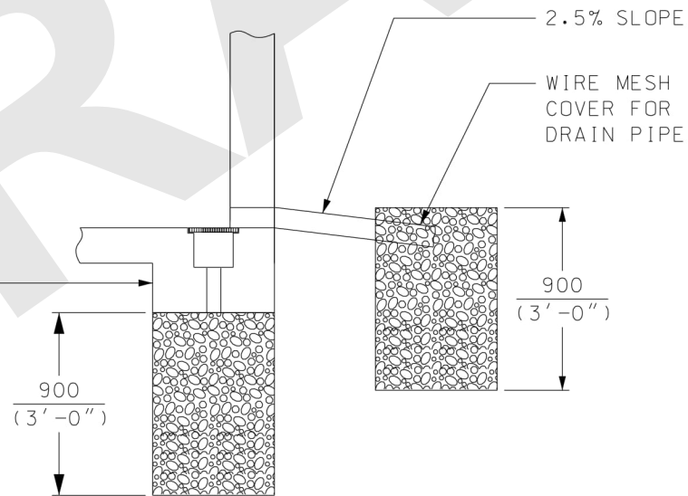
SECTION 'C-C'
