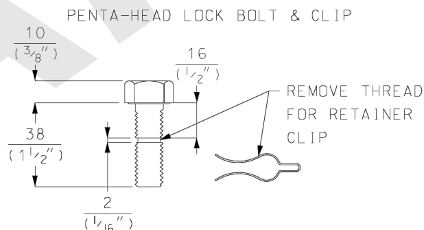
DETAIL 'H'
