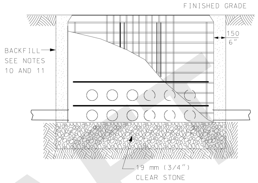
BOX SIDE VIEW INSTALLATION DETAIL
