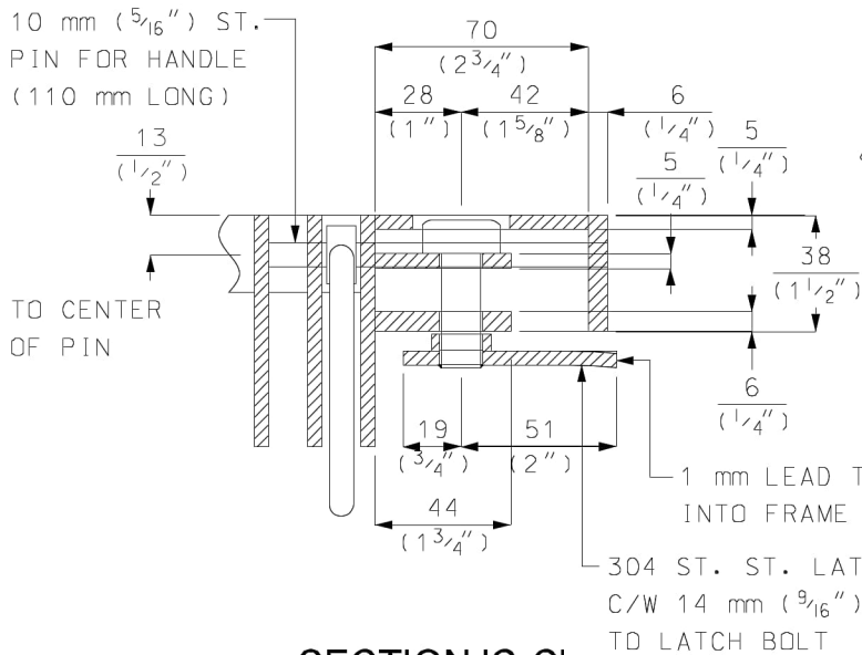
SECTION 'C-C'
