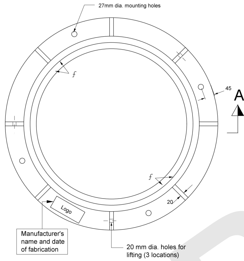
CABLE CHAMBER FRAME
