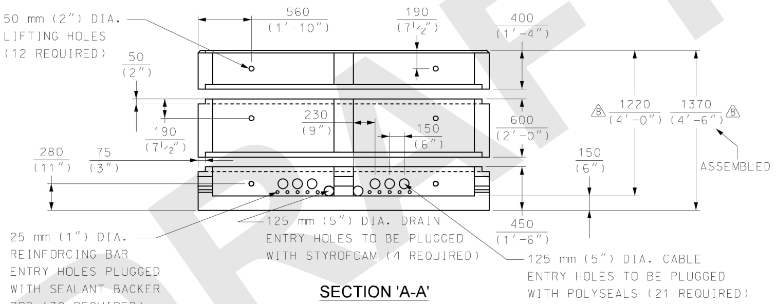
PLAN VIEW
