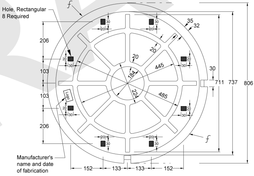
CABLE CHAMBER COVER
