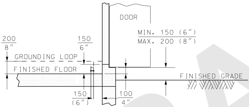
12 DETAIL 'A' DOOR AND GROUNDING DETAIL
