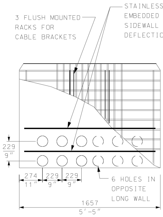
BOX SIDE VIEW ⚠️ LONG SIDEWALL
