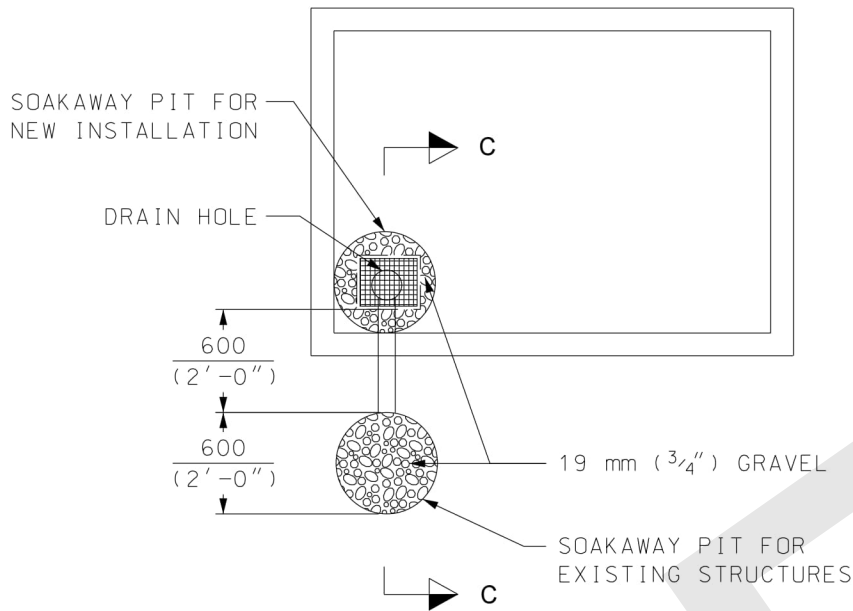
PLAN VIEW
