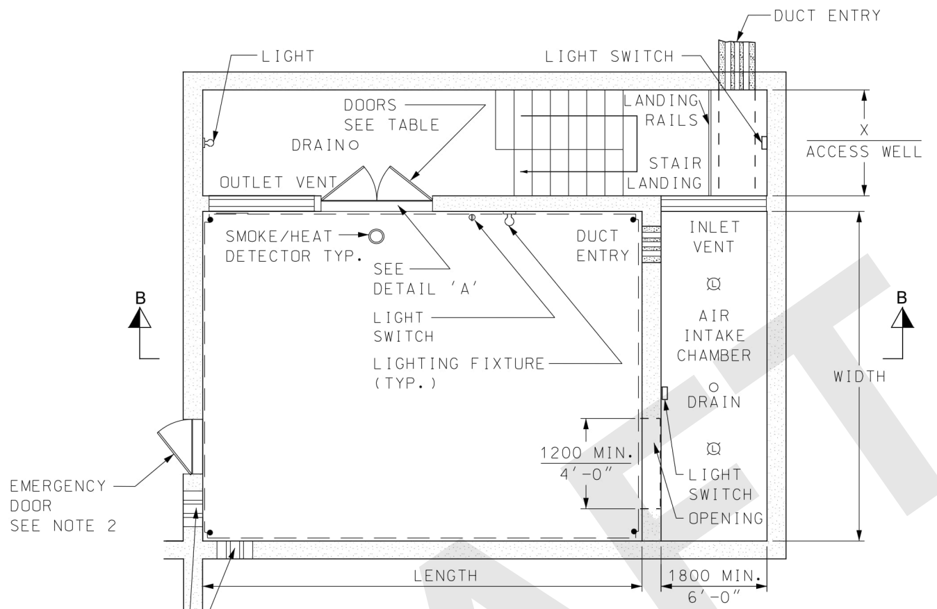
PLAN VIEW ALTERNATIVE VENTILATION
